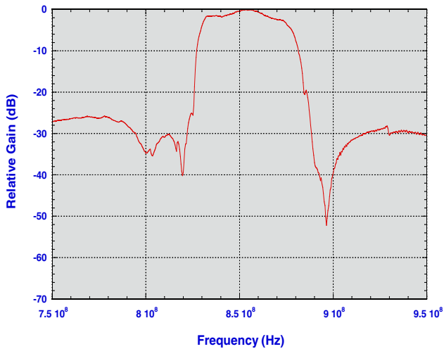
Clna-J Frequency Response
