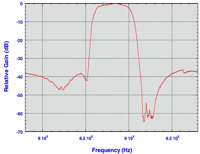
Clna-A Frequency Response
