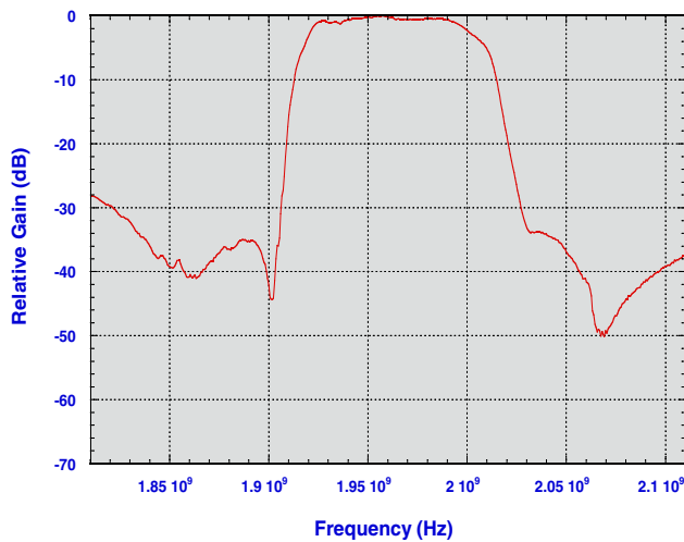
Clna-P Frequency Response
